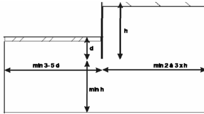
Suggestion for deformation analysis (based on Dutch situations): (K.J. Bakker, PAO course Damwanden)
